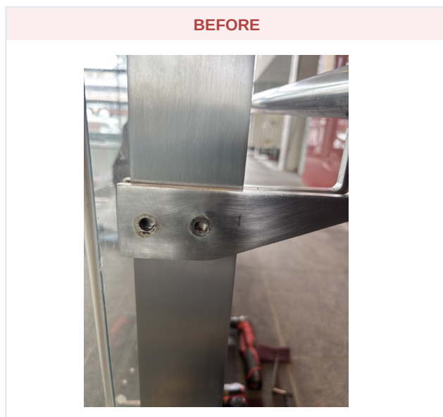
Handrail bracket / post connection - before restoration
