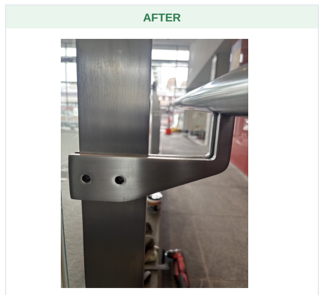
Handrail bracket / post connection - after restoration
